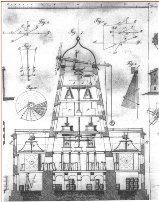
Drawing of an “English-American Windmill”
